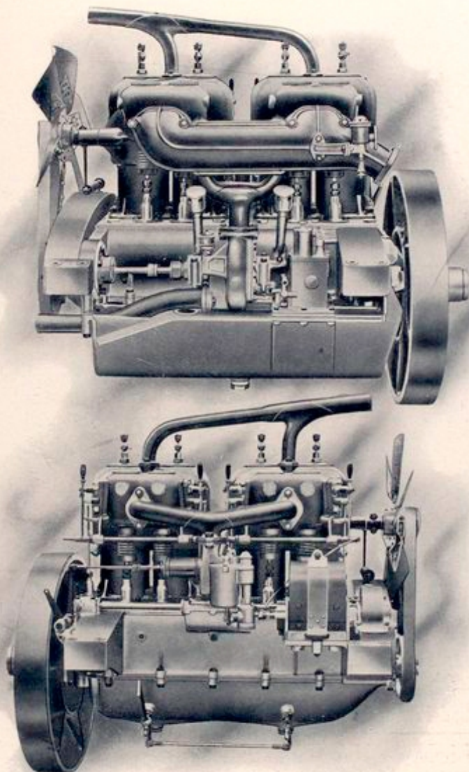
1909 Lorraine-Dietrich Engine
